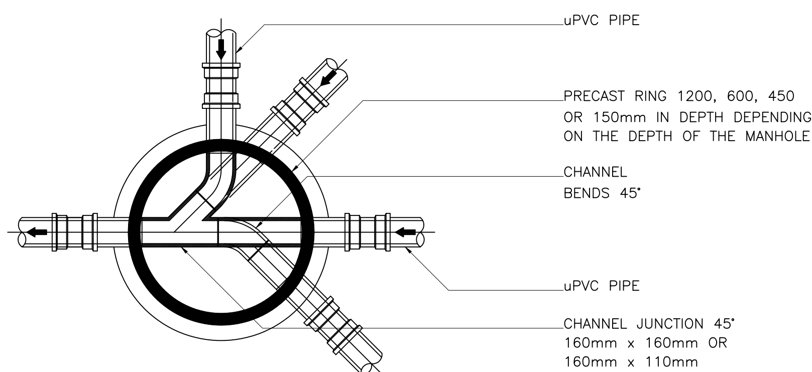
MANHOLE DETAILS 90° AND 45° CONNECTIONS
