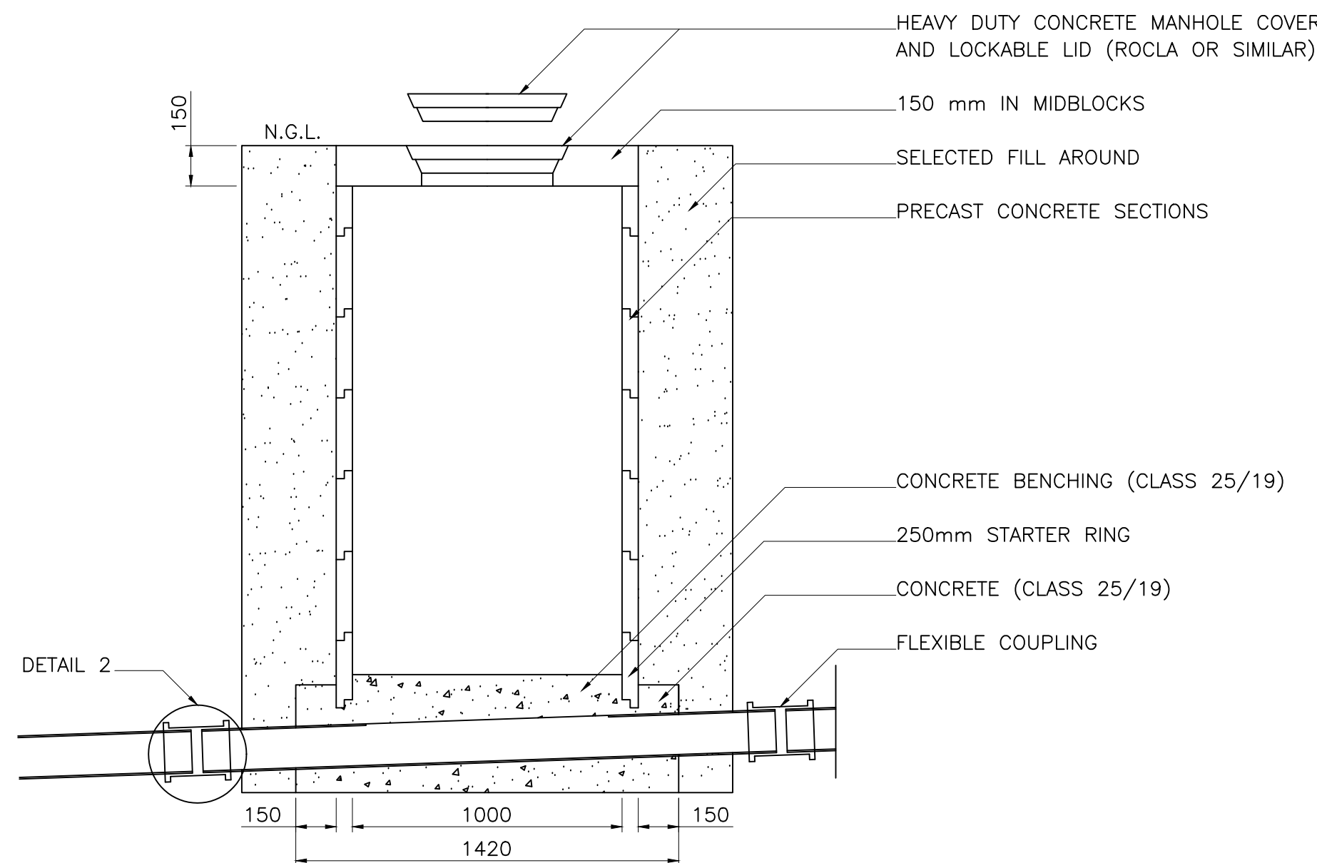
SECTION B-B
