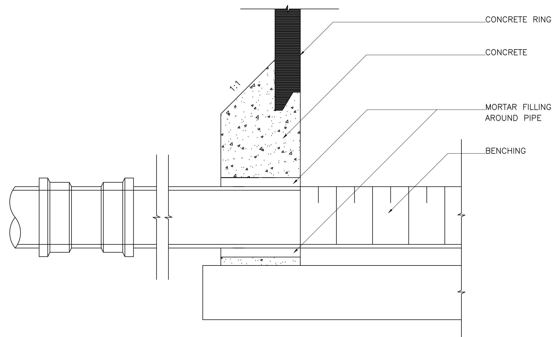
DETAIL 2
