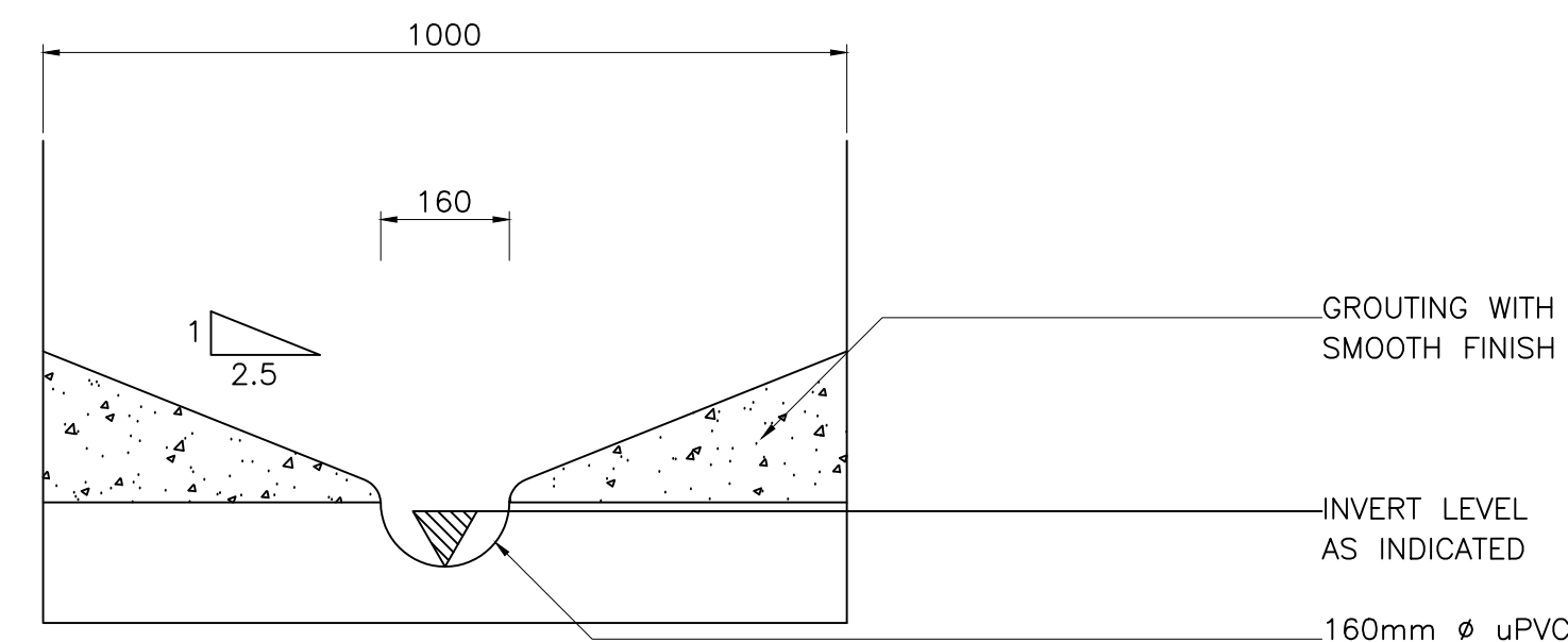
PROFILE IN MANHOLE
