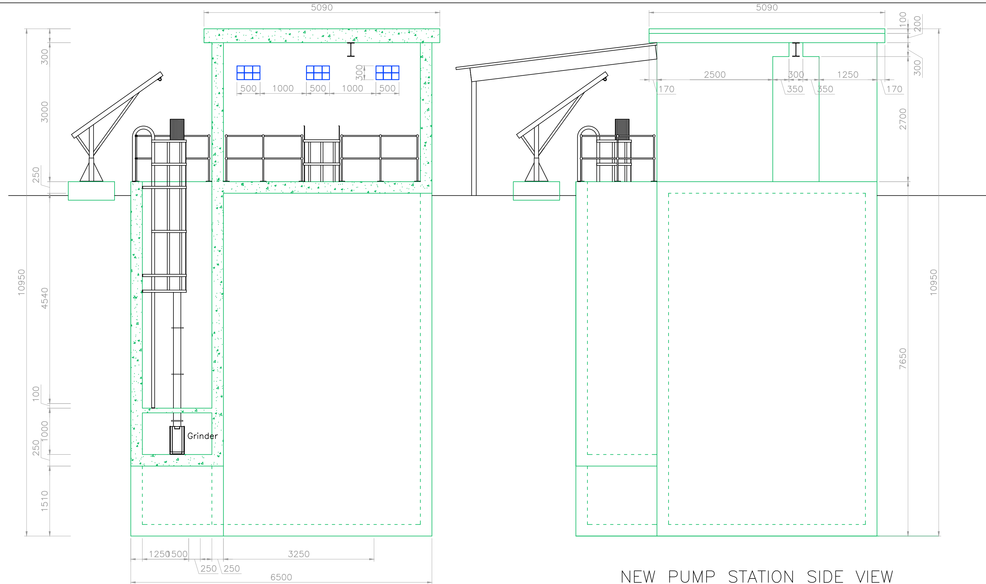
NEW PUMP STATION SIDE VIEW SCALE 1:50
