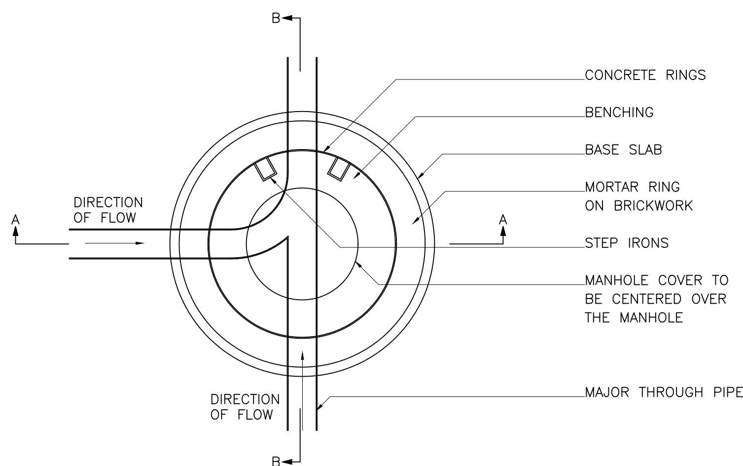
MANHOLE PLAN
