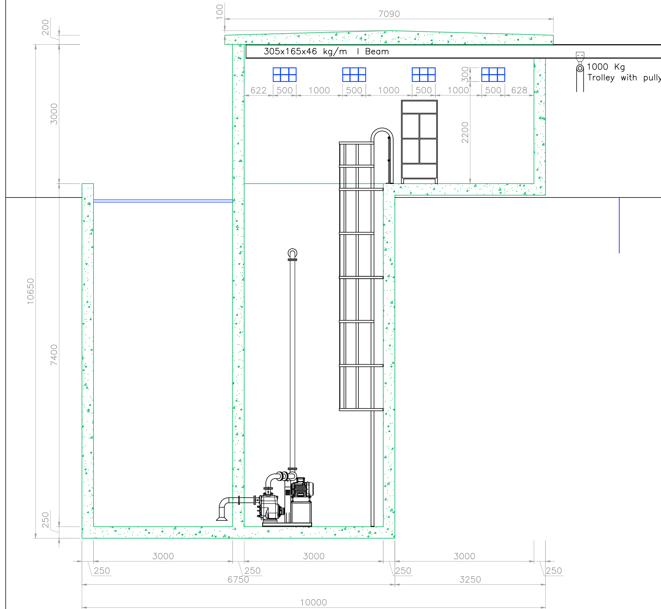
NEW PUMP STATION SECTION A-A SCALE 1:50
